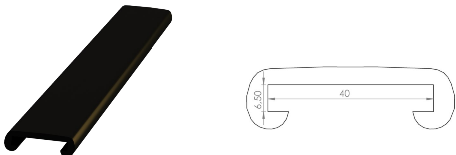
Dock finger's bumper profile
